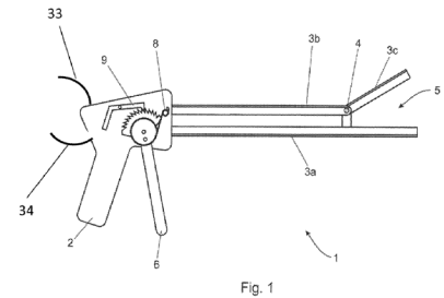
Fig. 1: Novel Stapler
